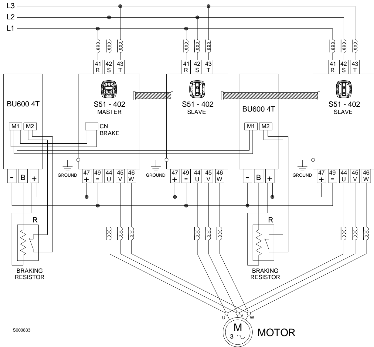
Figure 31: Power connections and location of two BU600 operating as slaves
