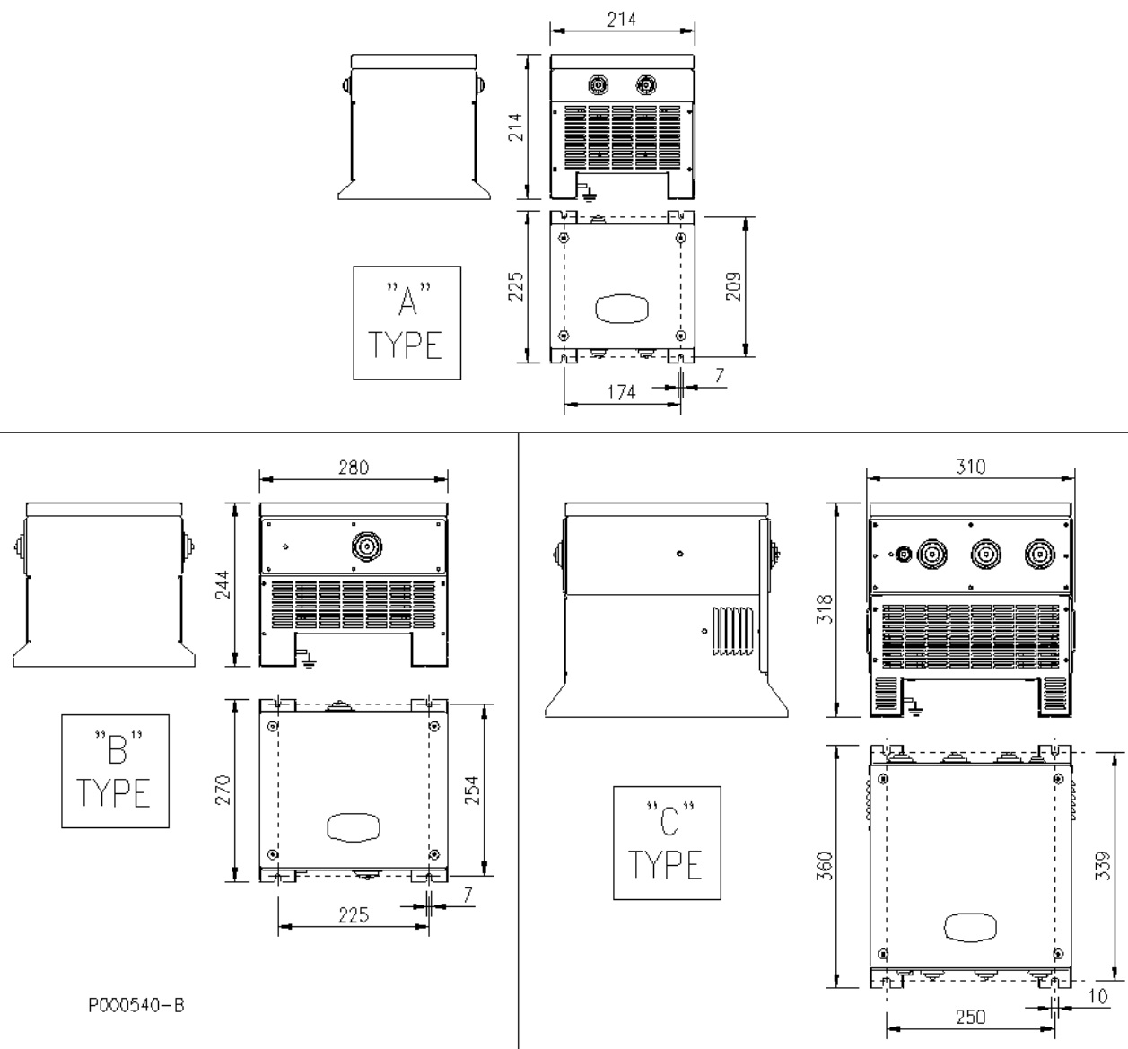
Figure 55: Mechanical features of three-phase inductors for Class 2T-4T in IP54 cabinet
