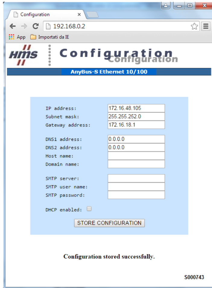
Figure 108: Internal webserver
