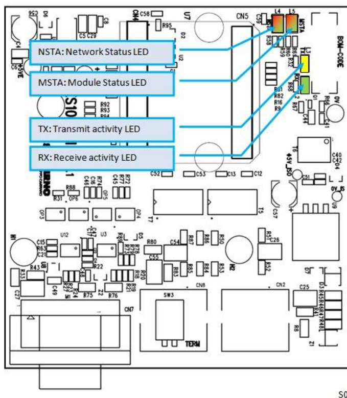
Figure 89: Position of the status LEDs on the B40 series board
