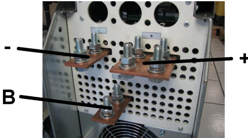
Figure 27: Power terminals
