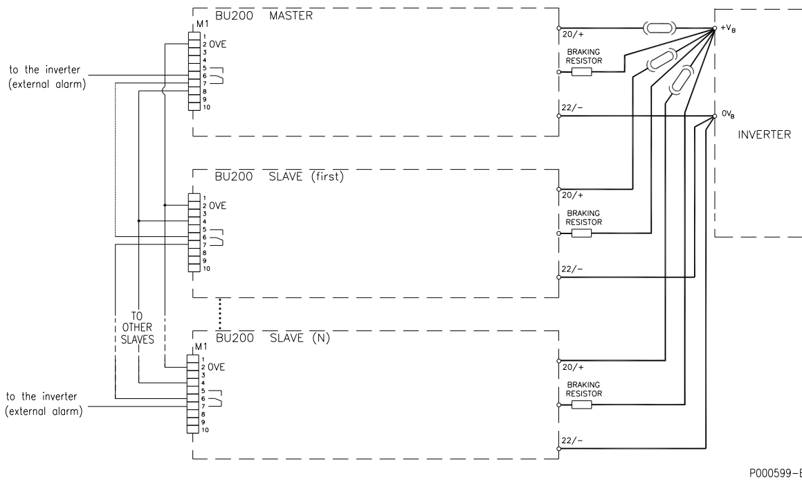
Figure 21: Master – Slave multiple connection
