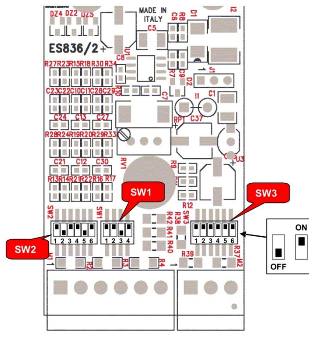
Figure 63: Positions of DIP-switches and their factory-setting
