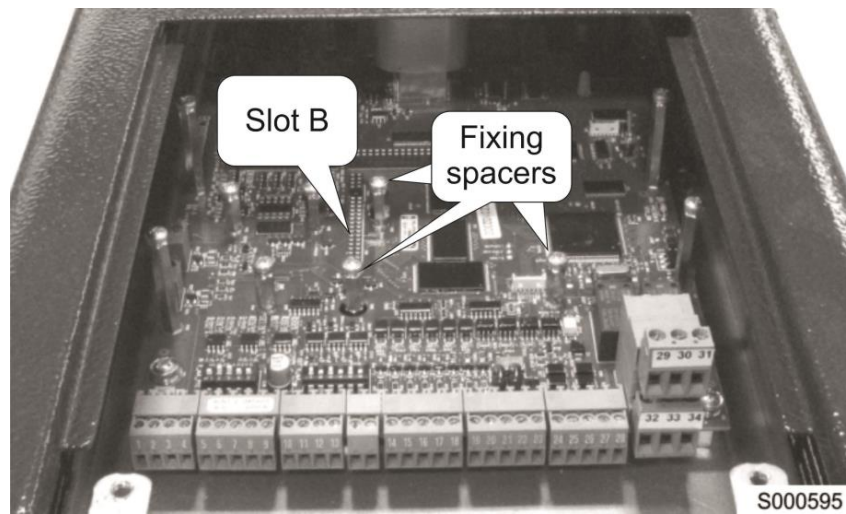
Figure 113: Position of the slot for ES919 board
