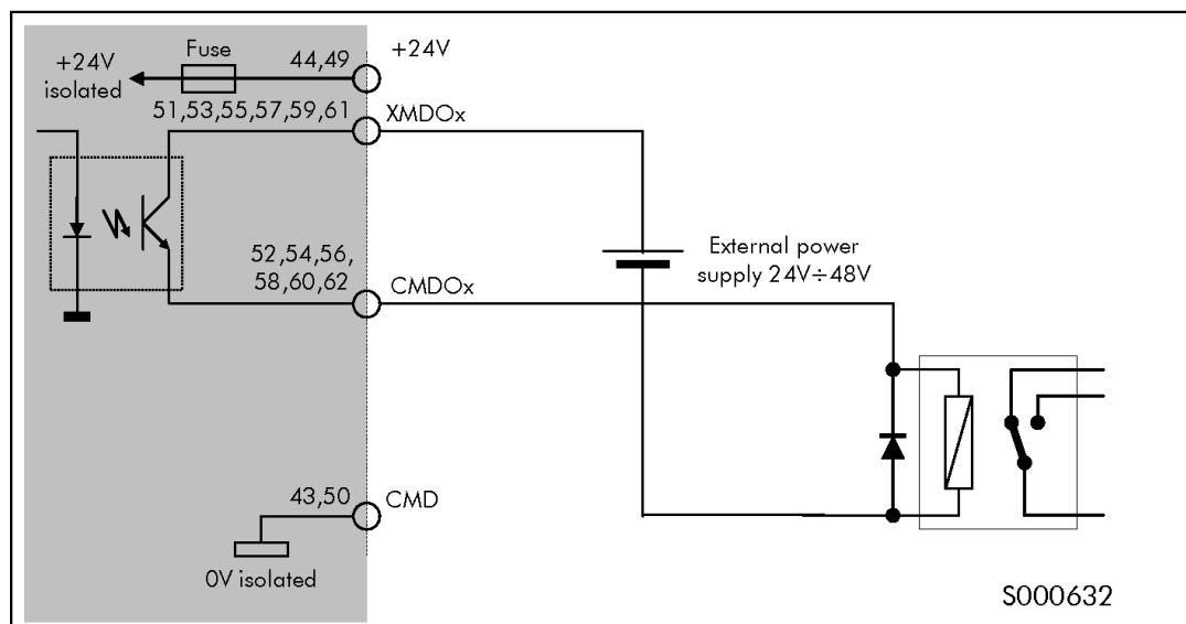
Figure 135: XMDOx output connection as PNP for relay command with external power supply
