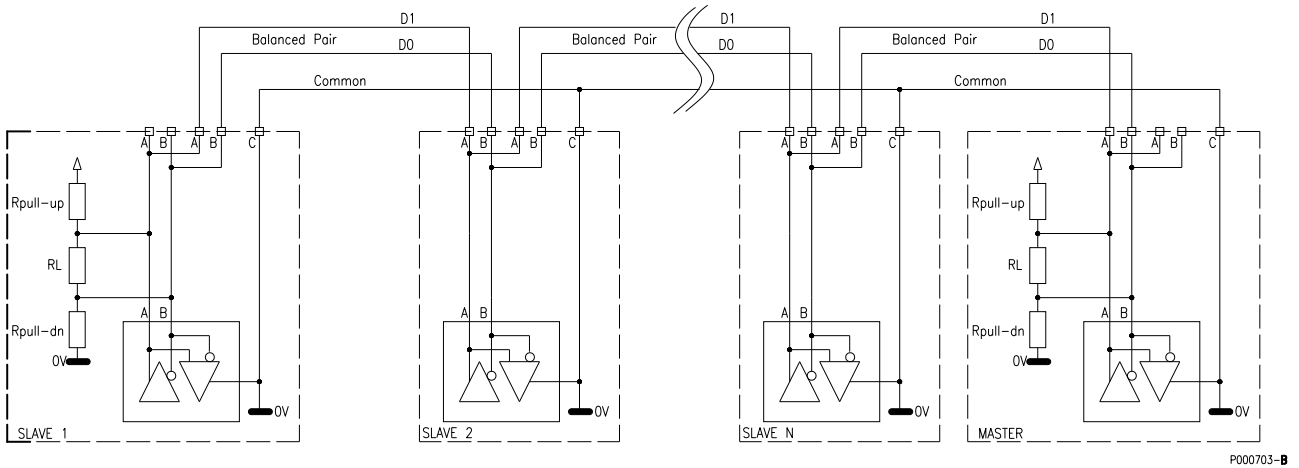
Figure 33: Recommended wiring diagram for “2-wire” MODBUS connection
