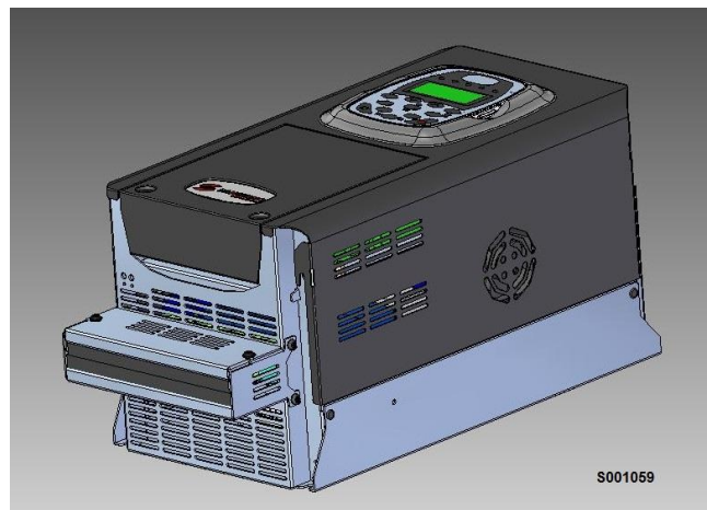
Figure 48: Example of a NEMA 1 Kit installed on a SINUS PENTA
