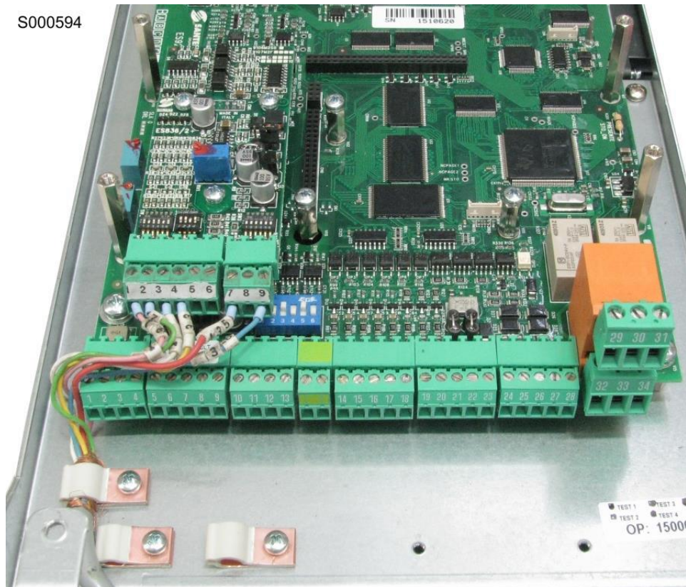
Figure 68: Wiring the encoder cable
