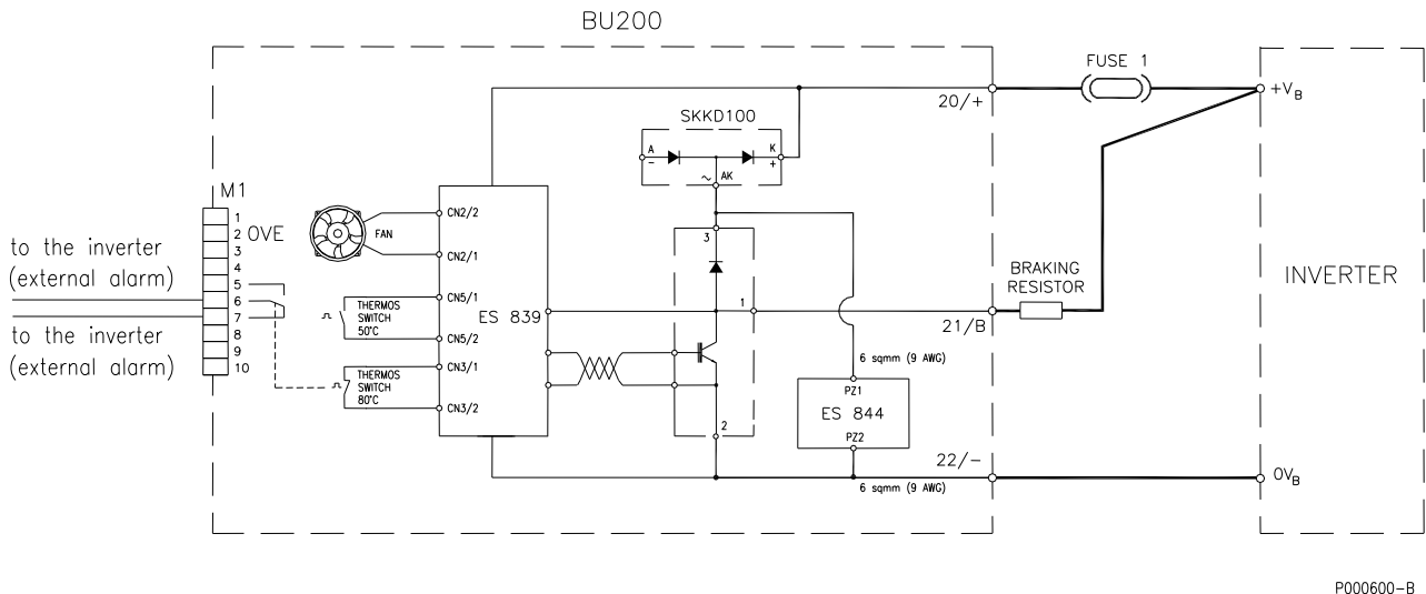
Figure 20: Connecting one BU200 to the inverter
