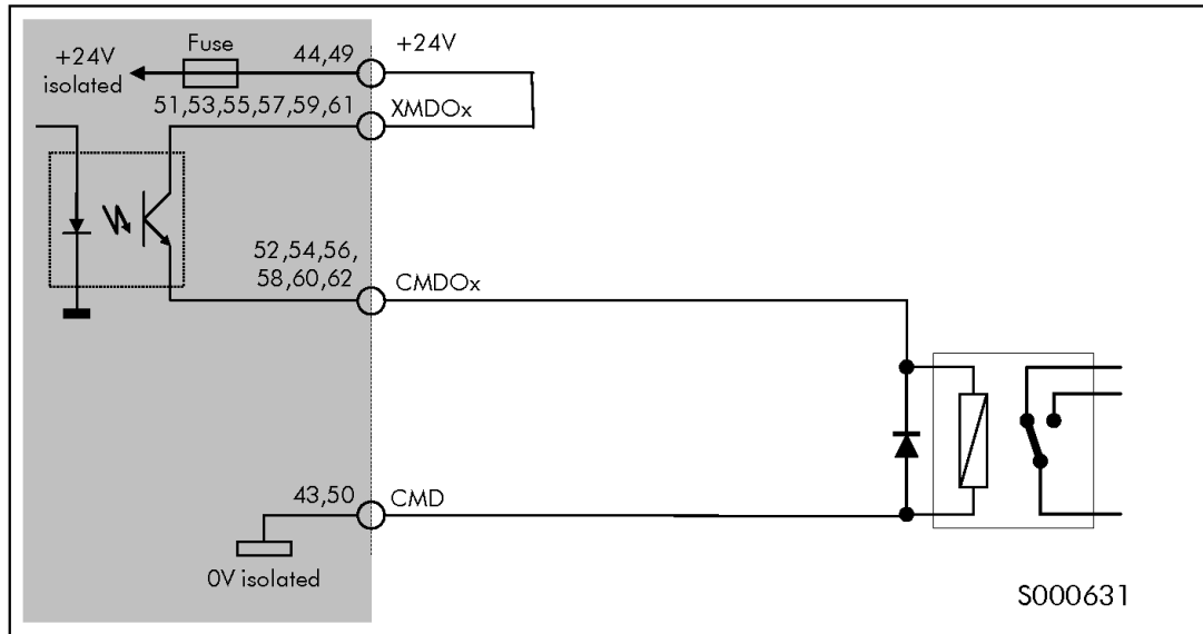
Figure 134: XMDOx output connection as PNP for relay command with internal power supply
