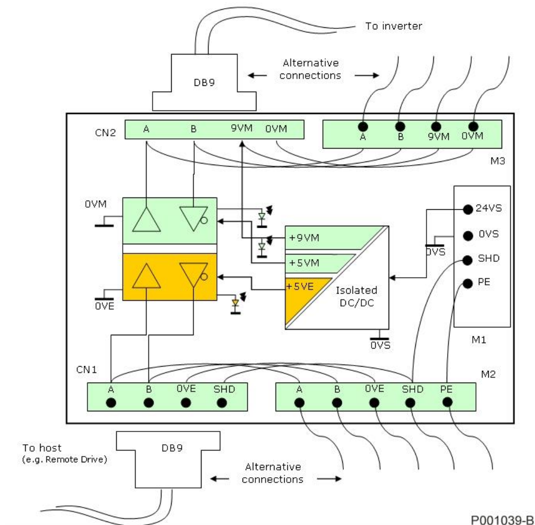
Figure 176: Block-diagram with 3-zone insulation
