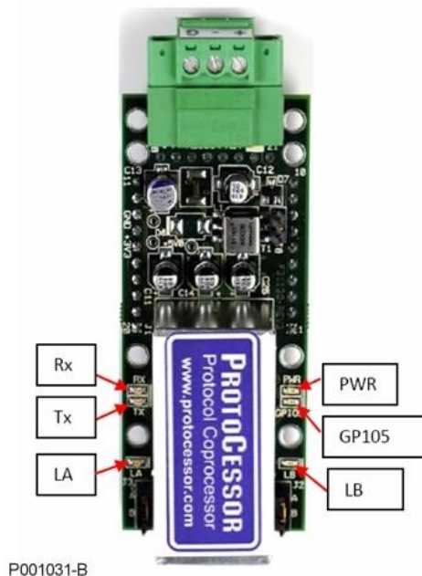
Figure 117: BACnet LEDs
