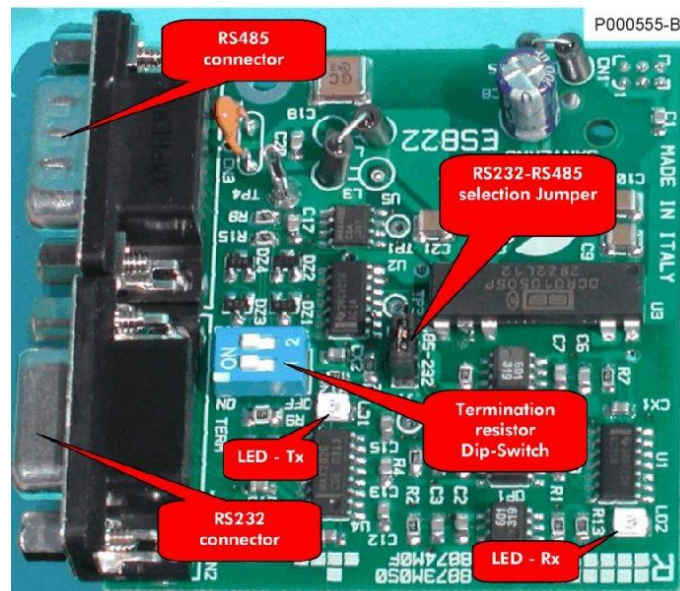
Figure 82: ES822 board
