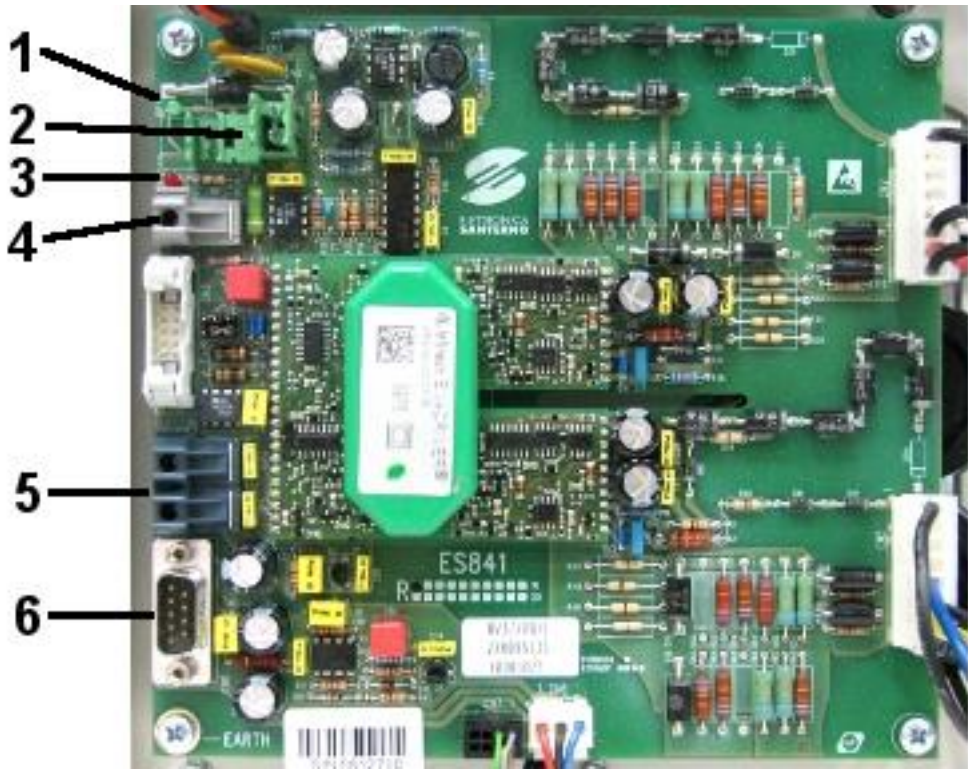
Figure 38: ES841 Unit gate board for the braking unit
