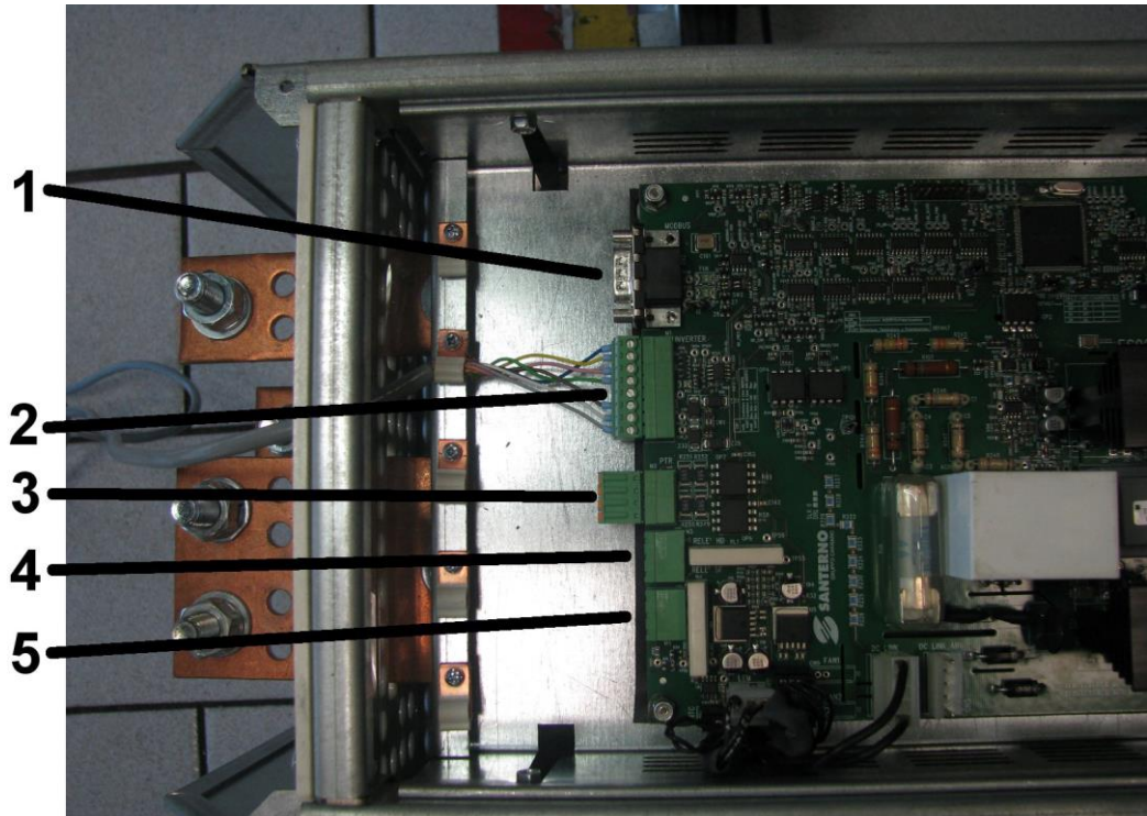
Figure 28: Signal terminals in the BU600
