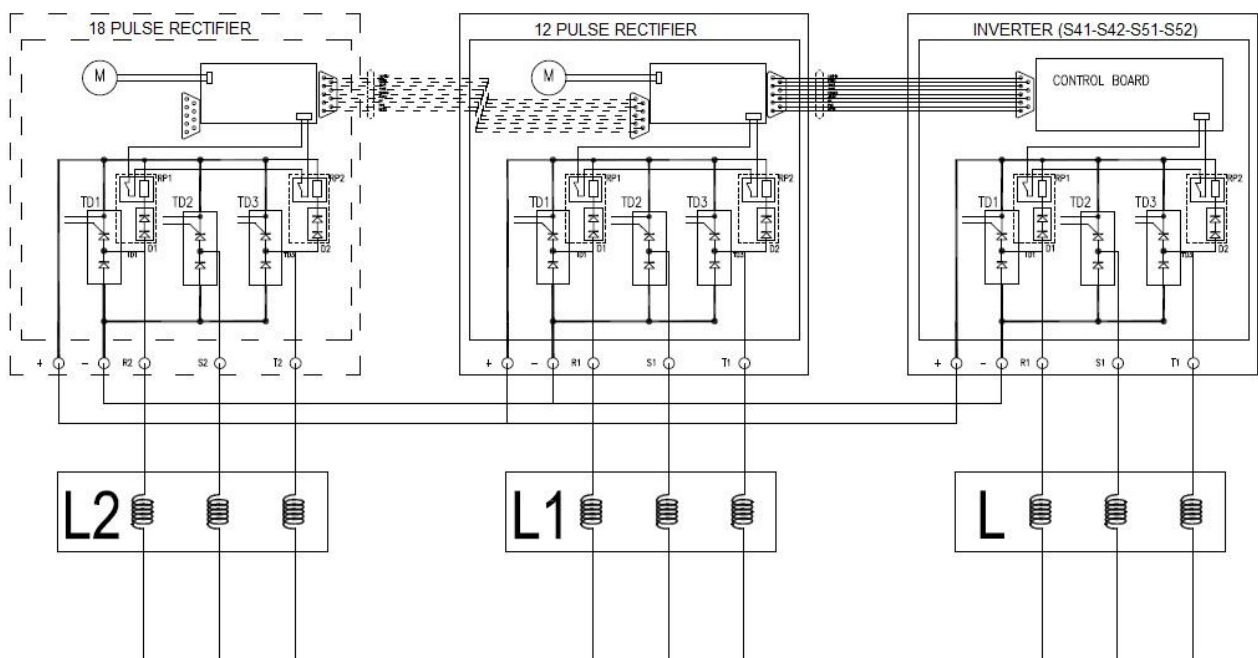
Figure 13: S41–S52 connections with 12- and 18-pulse SU465
