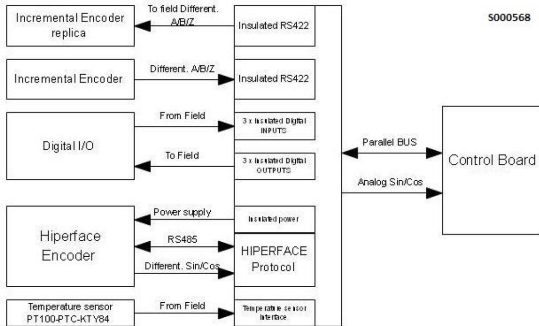
Figure 170: Block diagram of ES966 interface board
