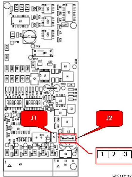
Figure 73: Location of the jumpers selecting the encoder supply voltage
