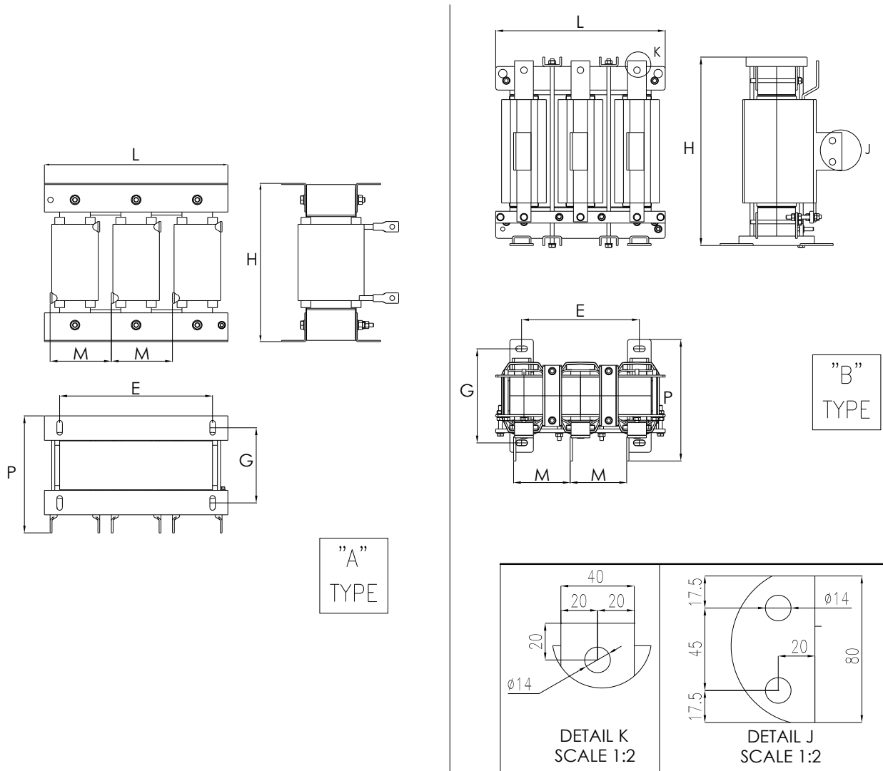
Figure 54: Mechanical features of the 3-phase du/dt inductors
