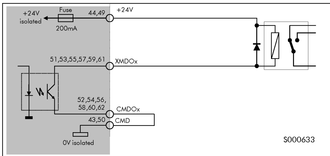
Figure 136: XMDOx output connection as NPN for relay command with internal power supply
